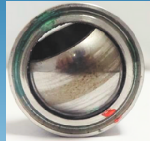
UNIFLON® MP after 30 million cycles
