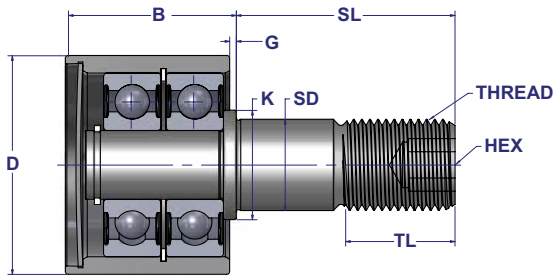
Ball Bearing (BB) Style
