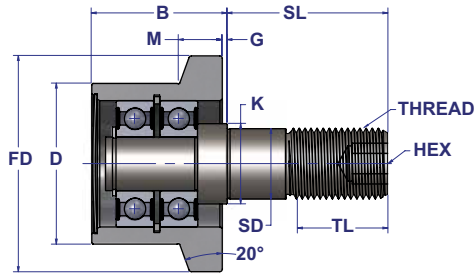
Ball Bearing (BB) Style
