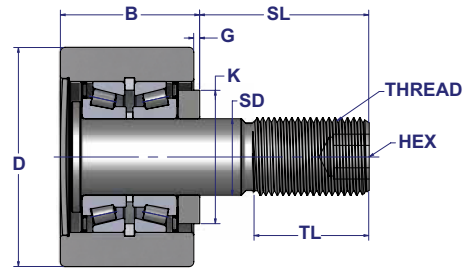
Tapered Roller Bearing (TRB) Style
