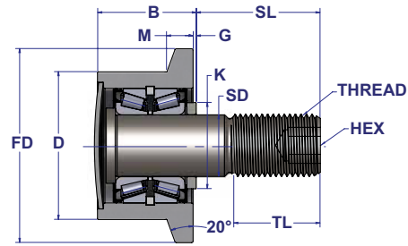
Tapered Roller Bearing (TRB) Style
